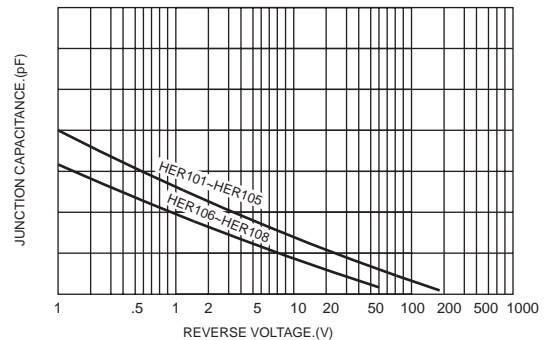
FIG.6-TYPICAL JUNCTION CHARACTERISTICS
