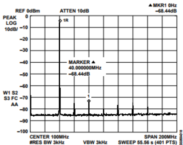
Figure 6. Four = 40 MHz, FCLK = 400 MSPS, WBSFDR
