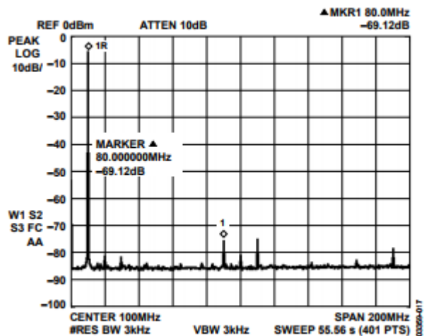
Figure 5. Four = 10 MHz, FCLK = 400 MSPS, WBSFDR
