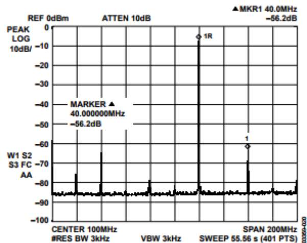
Figure 8. Four = 120 MHz, FCLK = 400 MSPS, WBSFDR
