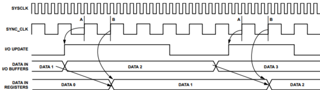
Figure 20. I/O Synchronization Timing Diagram
