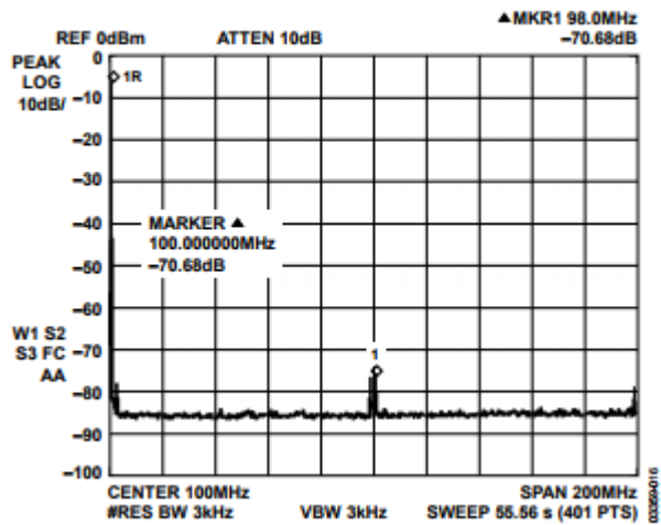
Figure 4. Four = 1 MHz FCLK = 400 MSPS, WBSFDR
