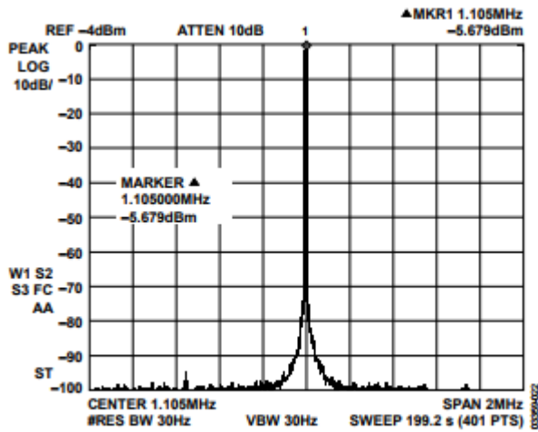
Figure 10. F_{out} = 1.1 \text{ MHz} , F_{CLK} = 400 \text{ MSPS} , NBSFDR, \pm 1 \text{ MHz}
