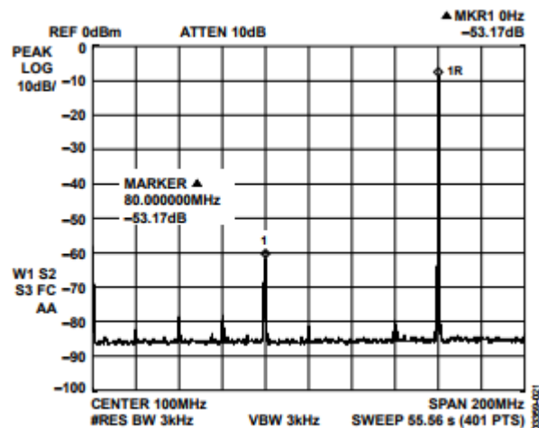
Figure 9. Four = 160 MHz, FCLK = 400 MSPS, WBSFDR
