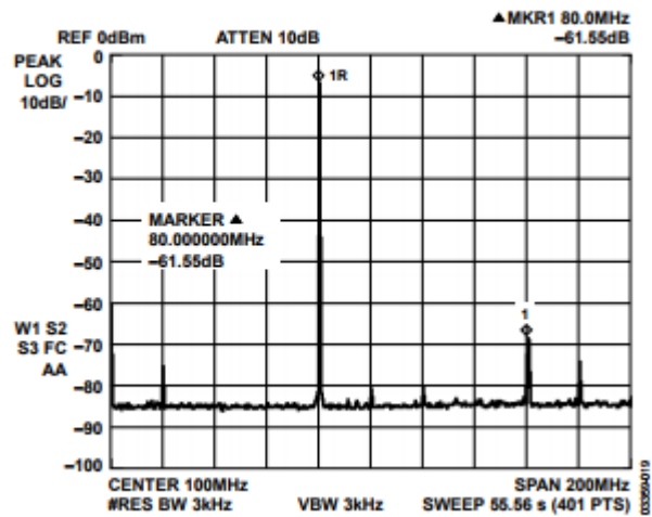
Figure 7. Four = 80 MHz FCLK = 400 MSPS, WBSFDR
