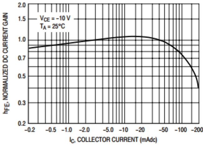
Figure 19. Normalized DC Current Gain
