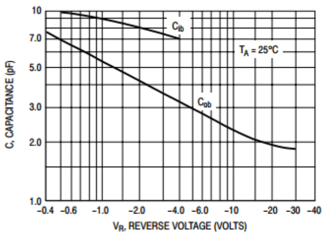
Figure 23. Capacitances
