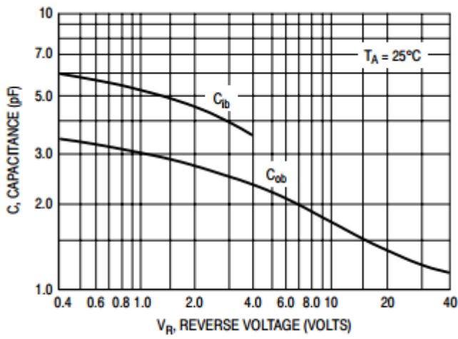
Figure 17. Capacitances
