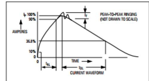
Figure 3b. Human Body Current Waveform
