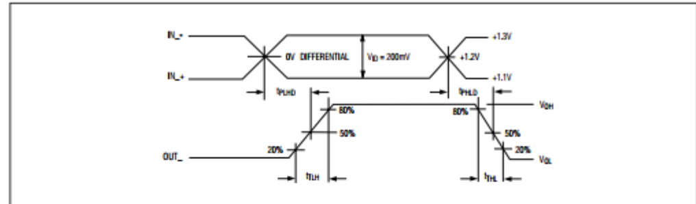
Figure 2. Receiver Propagation Delay and Transition Time Waveforms
