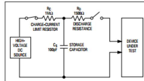
Figure 3a. Human Body ESD Test Modules
