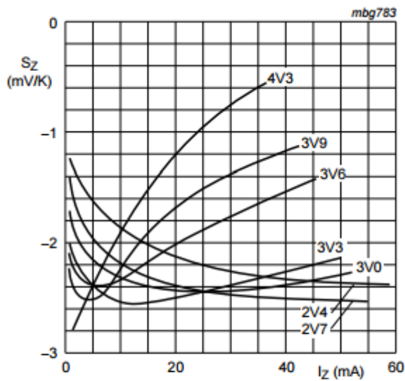
BZX84-A/B/C2V4 to BZX84-A/B/C4V3 T_j = 25\text{ }^\circ\text{C to }150\text{ }^\circ\text{C}
