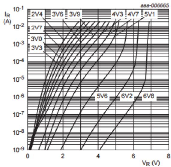
BZX84-A/B/C2V4 to BZX84-A/B/C6V8 T_{amb} = 25\text{ }^\circ\text{C}
