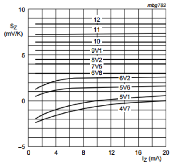
BZX84-A/B/C4V7 to BZX84-A/B/C12 T_j = 25\text{ }^\circ\text{C to }150\text{ }^\circ\text{C}
