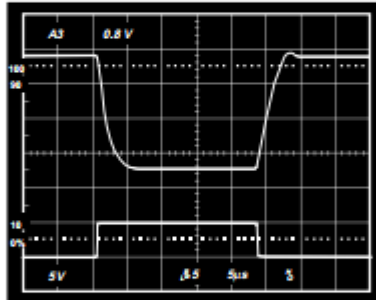
Figure 21. Transmitter Output Loaded Slew Rate
