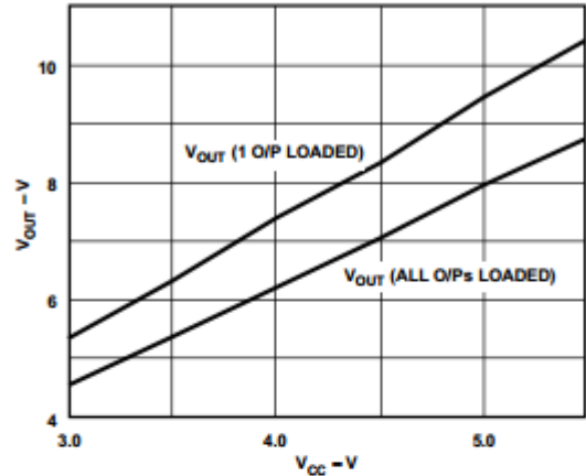
Figure 17. Transmitter Output Voltage vs. V_{CC}
