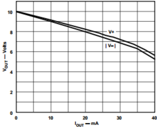
Figure 15. Charge Pump V_+ , V_- vs. Current
