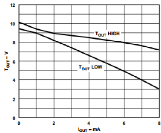
Figure 18. Transmitter Output Voltage vs. Current
