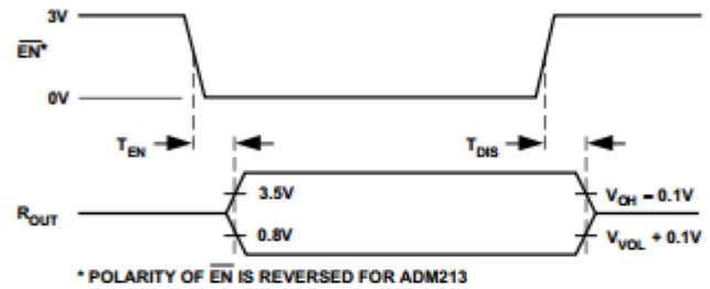
Figure 25. Enable Timing
