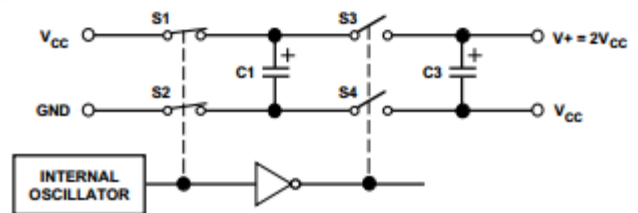
Figure 23. Charge-Pump Voltage Doubler
