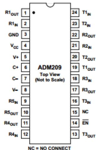
Figure 9. ADM209 DIP/SOIC/SSOP Pin Configuration
