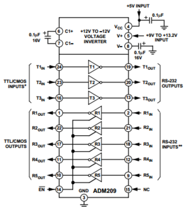
Figure 10. ADM209 Typical Operating Circuit
