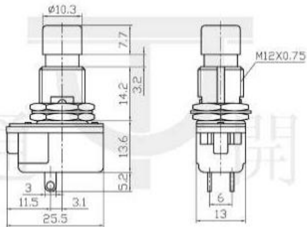
Outline Drawing
